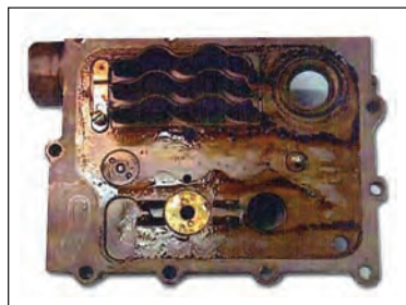
A level 3 vaporizer, BEFORE using REVGAS
